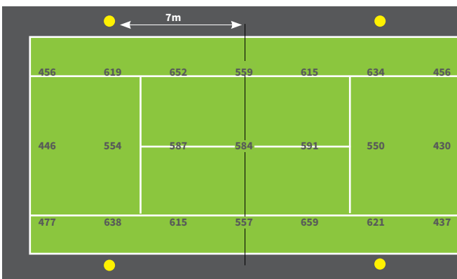
Simulation 2 - 568 Lux
