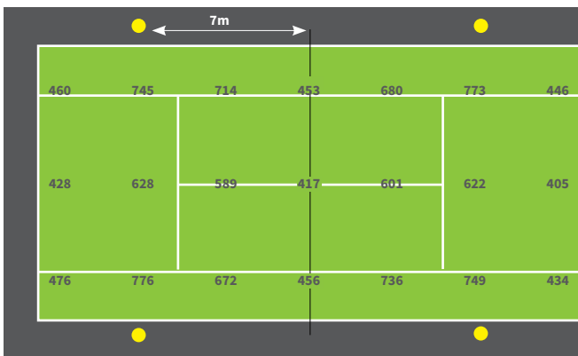
Simulation 1 - 594 Lux
